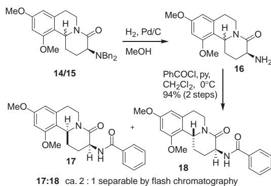
Scheme 4. Debenzylation of 14 and 15 and their conversion to benzamide derivatives 17 and 18 .
